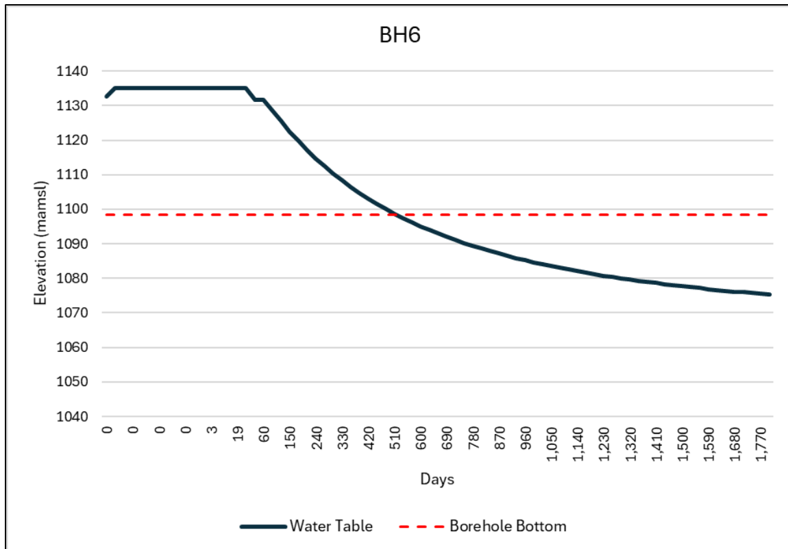
Figure 7.4: Simulated groundwater level drawdown in borehole BH6
