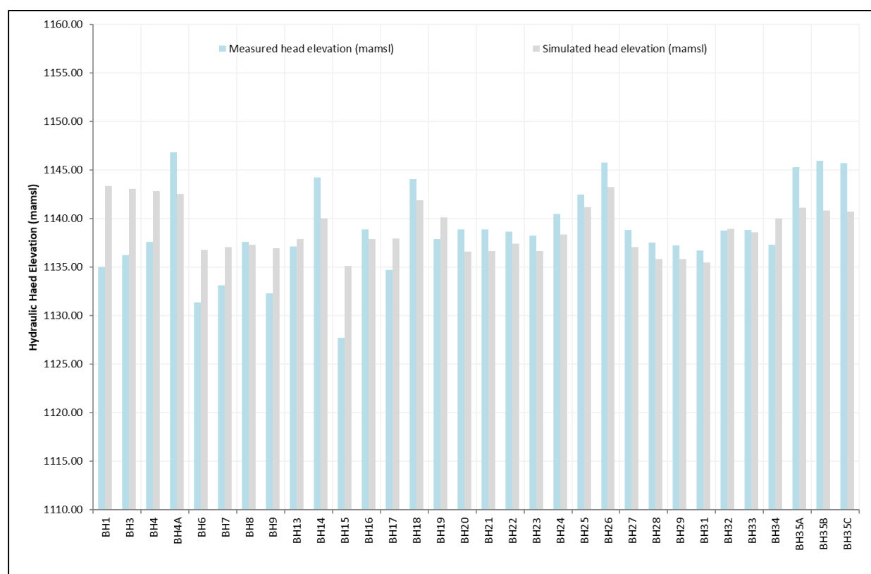
Figure 5.4: Correlation between simulated and observed groundwater levels
