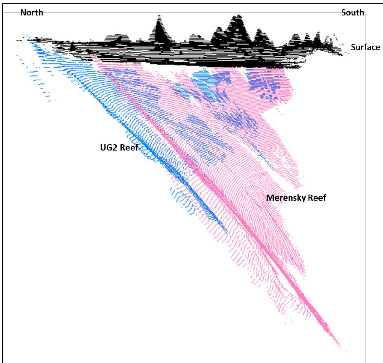
Figure 5.1: 3-Dimensional mined-out model
