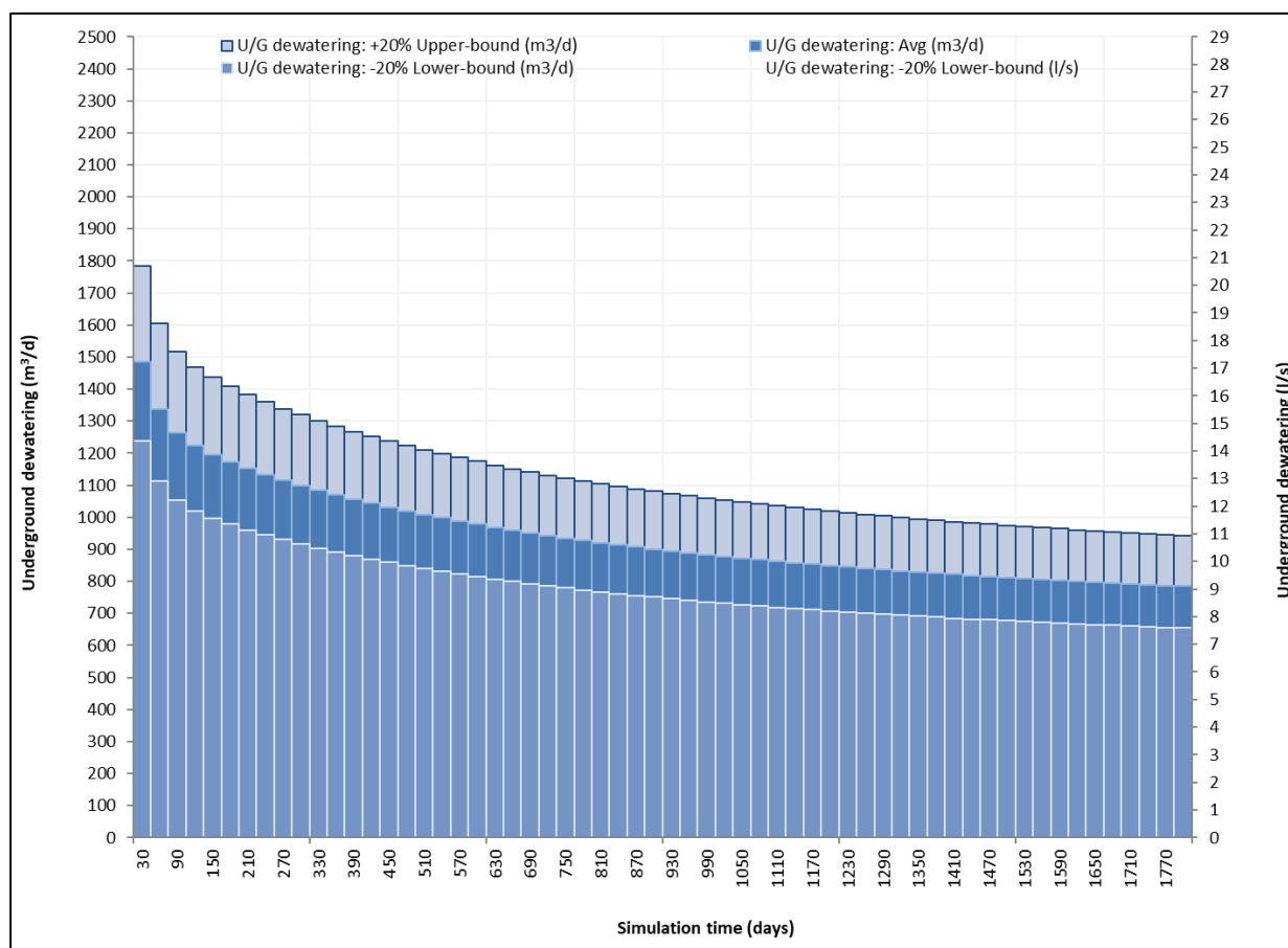
Figure 7.2: Estimated groundwater inflow volume – Block B
