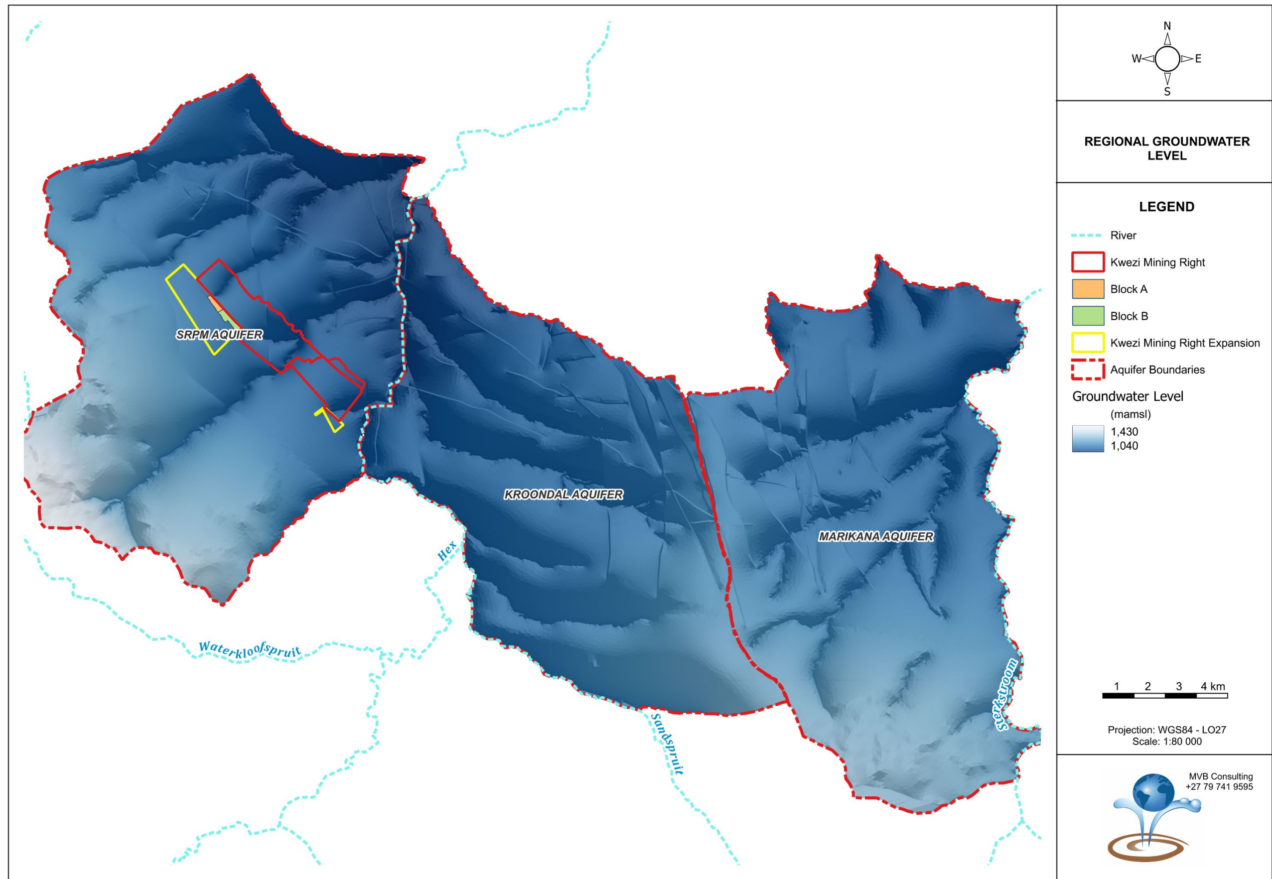
Figure 4.5: Regional groundwater gradients and aquifer boundaries
