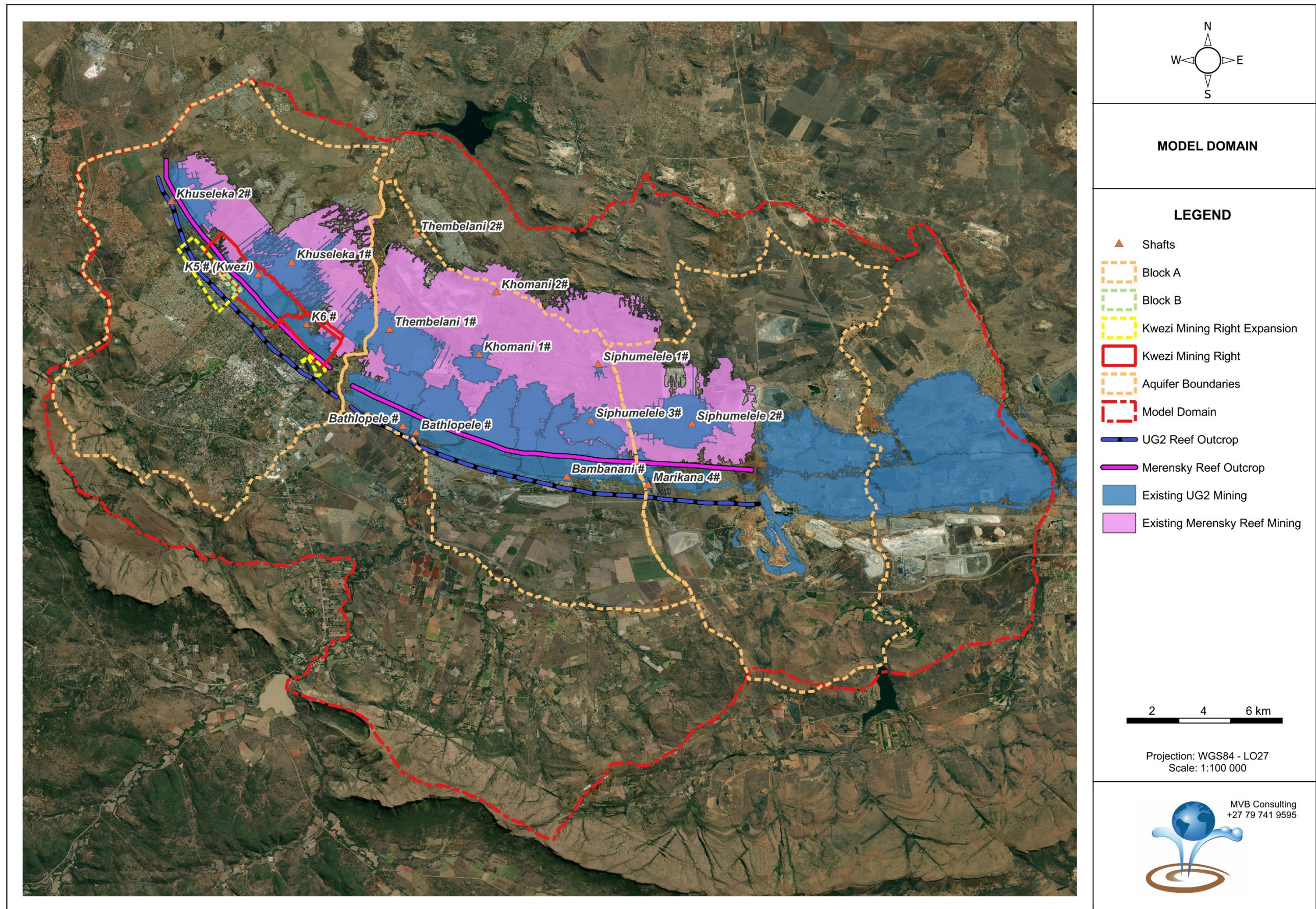
Figure 6.1: Model domain
