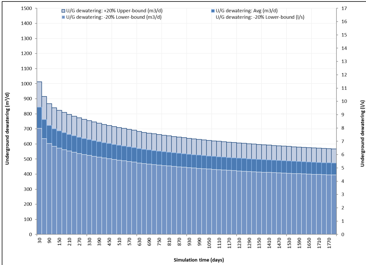
Figure 7.1: Estimated groundwater inflow volume – Block A
