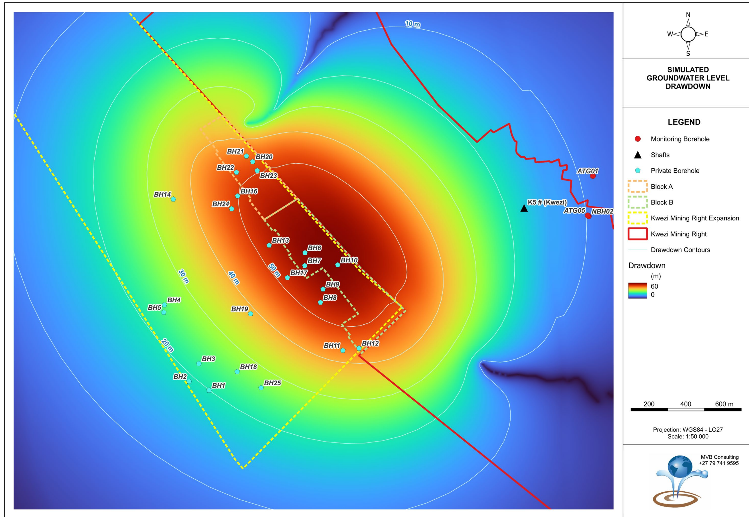
Figure 7.3: Simulated groundwater level drawdown within the Kwezi mining extension
