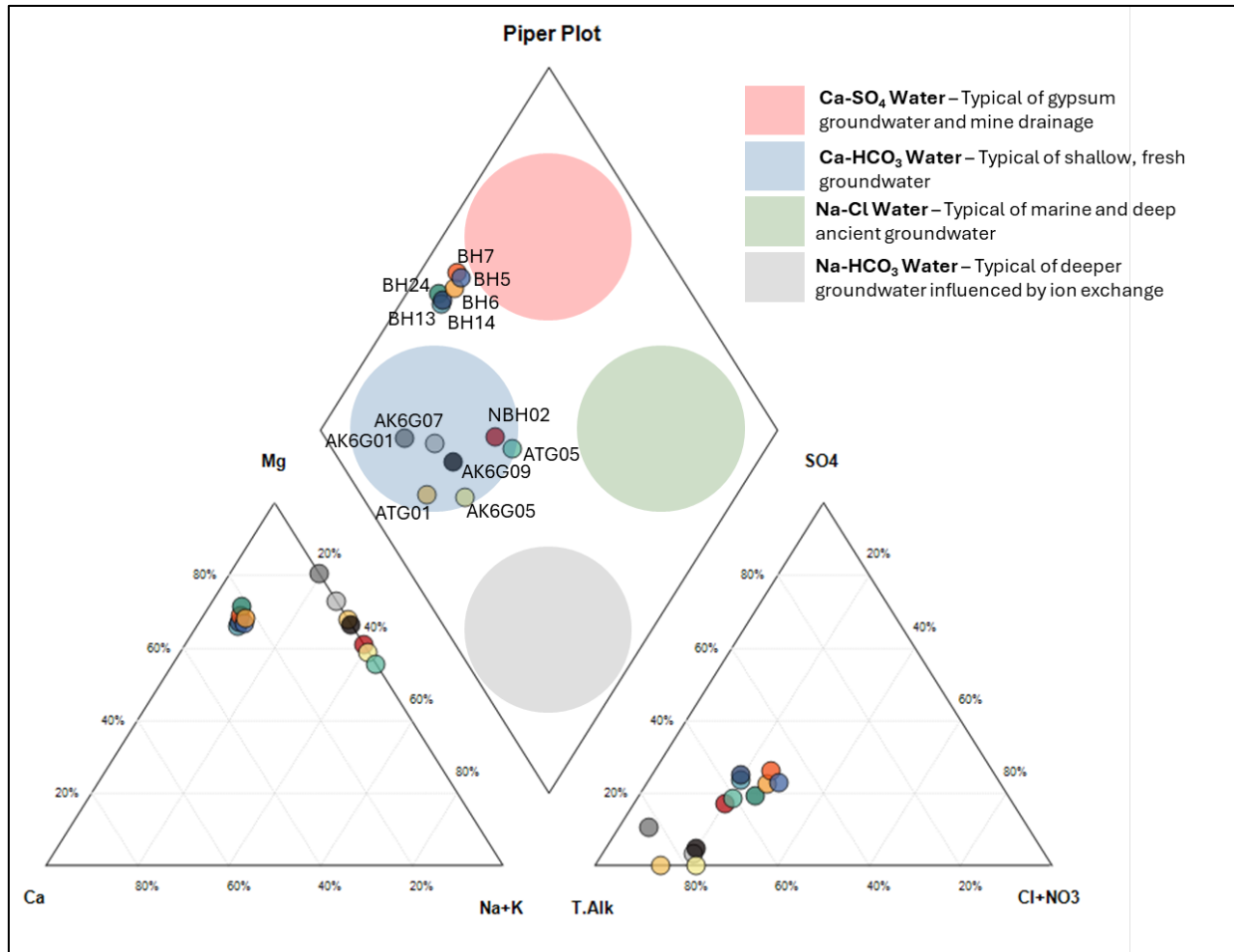
Figure 4.7: Piper diagram for the Kwezi region groundwater samples
