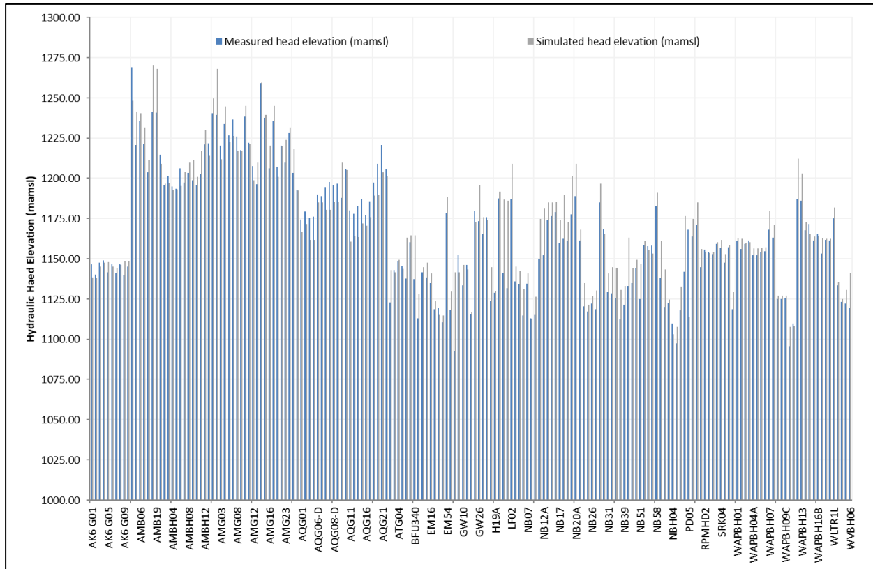
Figure 6.2: Correlation between simulated and observed groundwater levels
