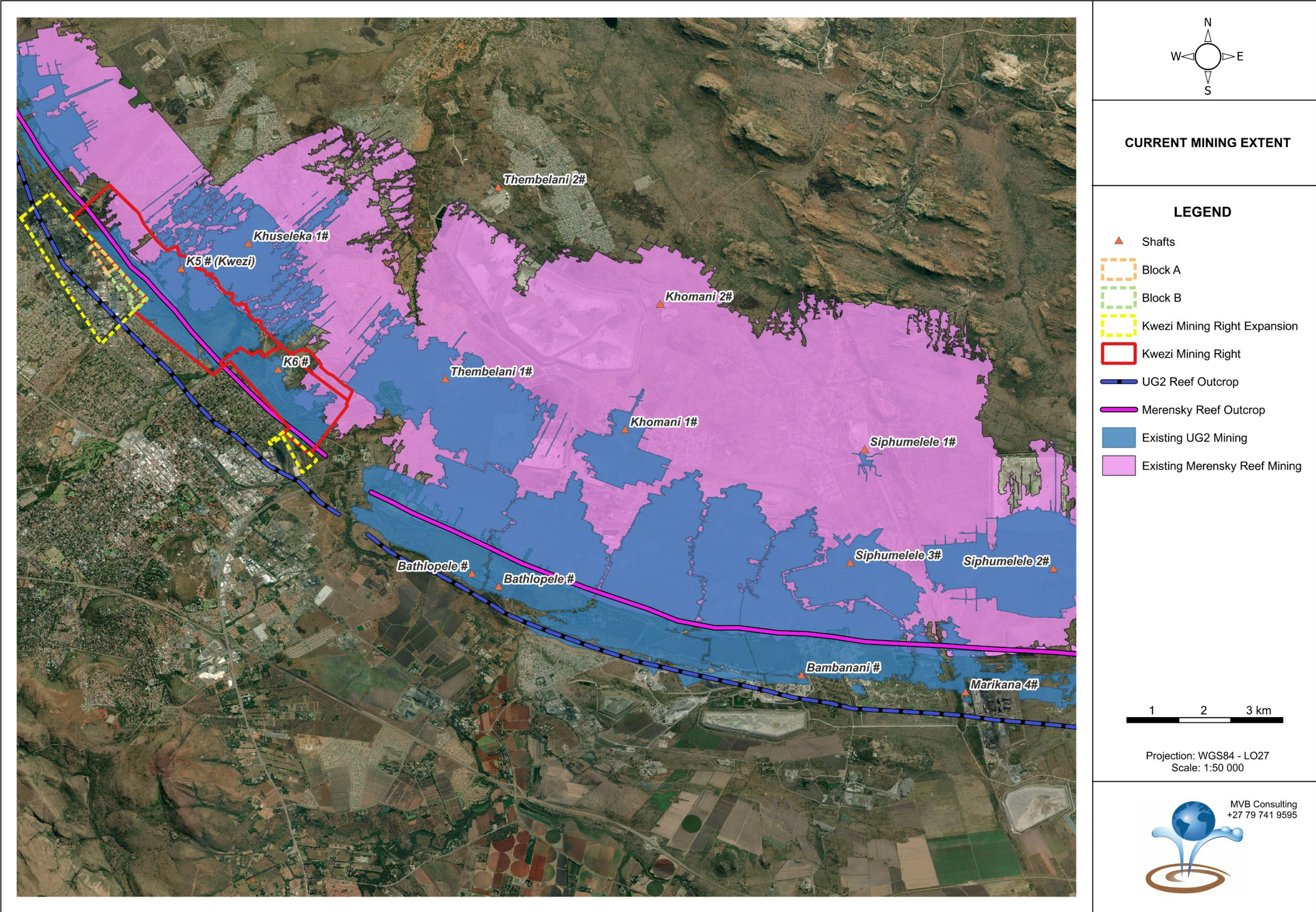
Figure 5.2: Underground mining extent
