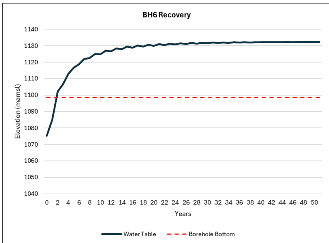
Figure 7.5: Simulated groundwater level recovery in borehole BH6
